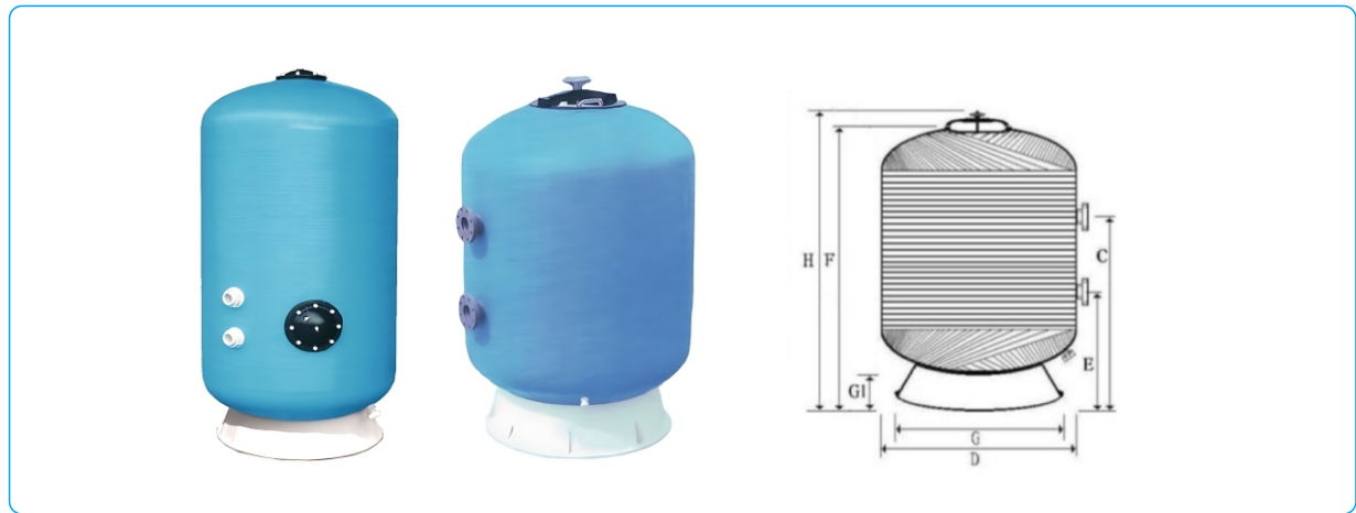
FA/DFB深層過濾砂缸 FA/DFB Series- Deep filter sand cylinder
